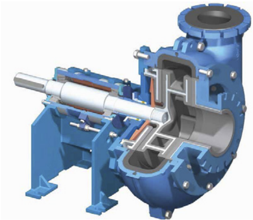
HR wet end single adjust, HM wet end double adjust
