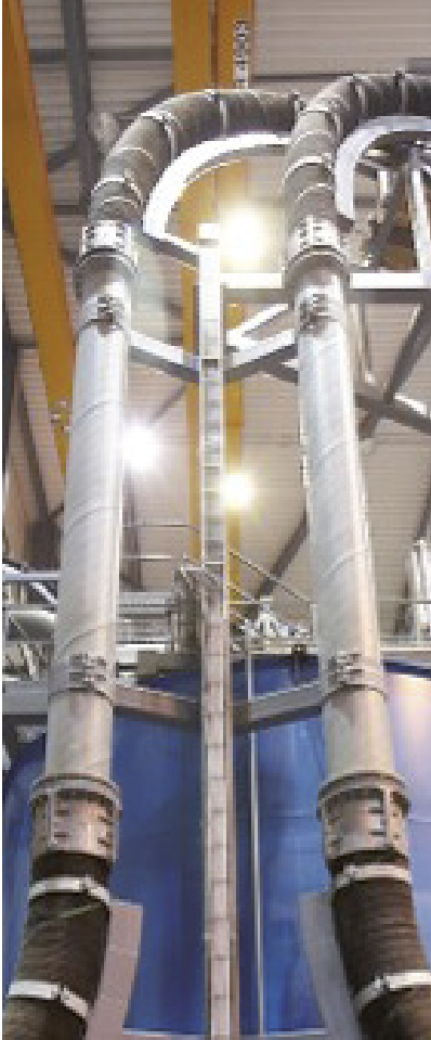
Picture 1: Material handling hose and rubber lined steel pipe
