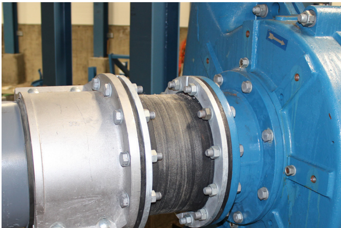
Picture 5: Rubber lined steel pipe and compensator
