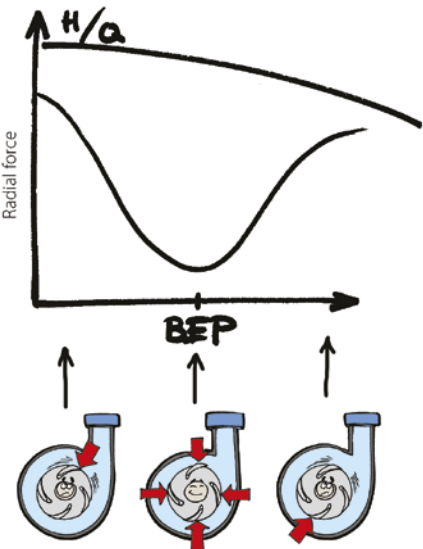
Over BEP operation
