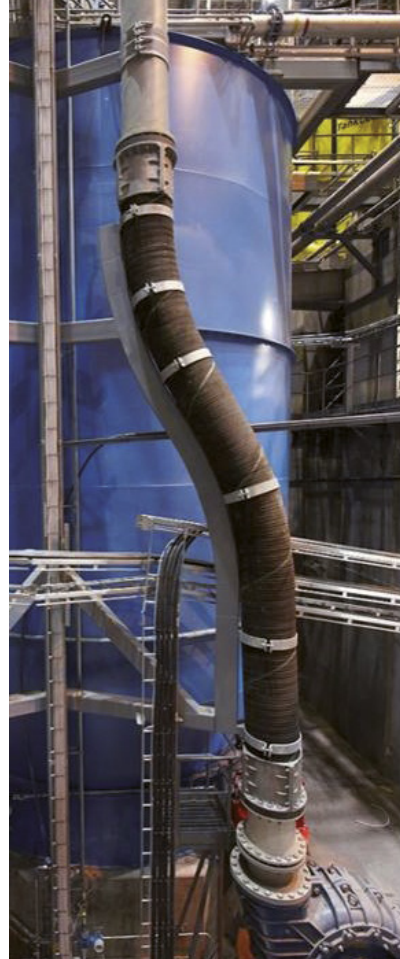
Picture 2: Material handling hose with support beam and clamps
