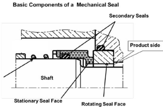
Figure 8: Basic mechanical seal components
