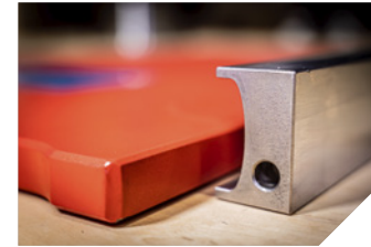
Toggle plate and toggle seat
