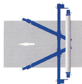
The belt conductor has guided the belt back on track.
