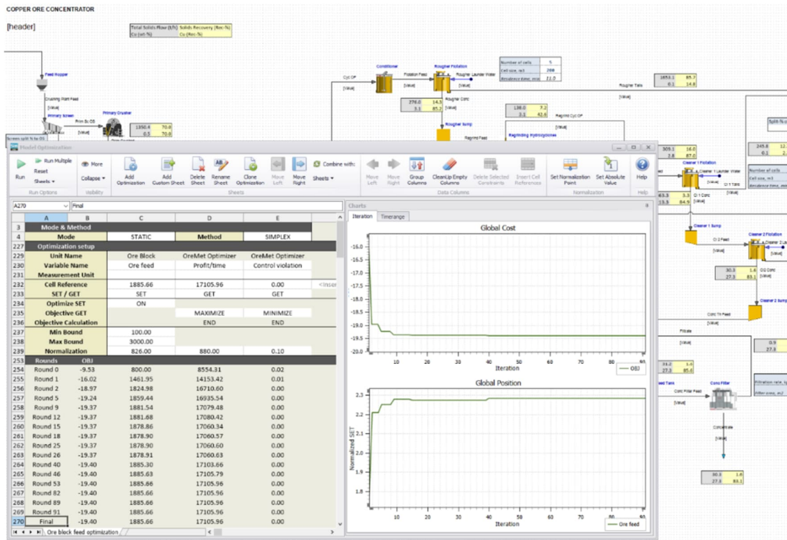
Figure 3. The new Model Optimization tool allows optimizing of process performance.
