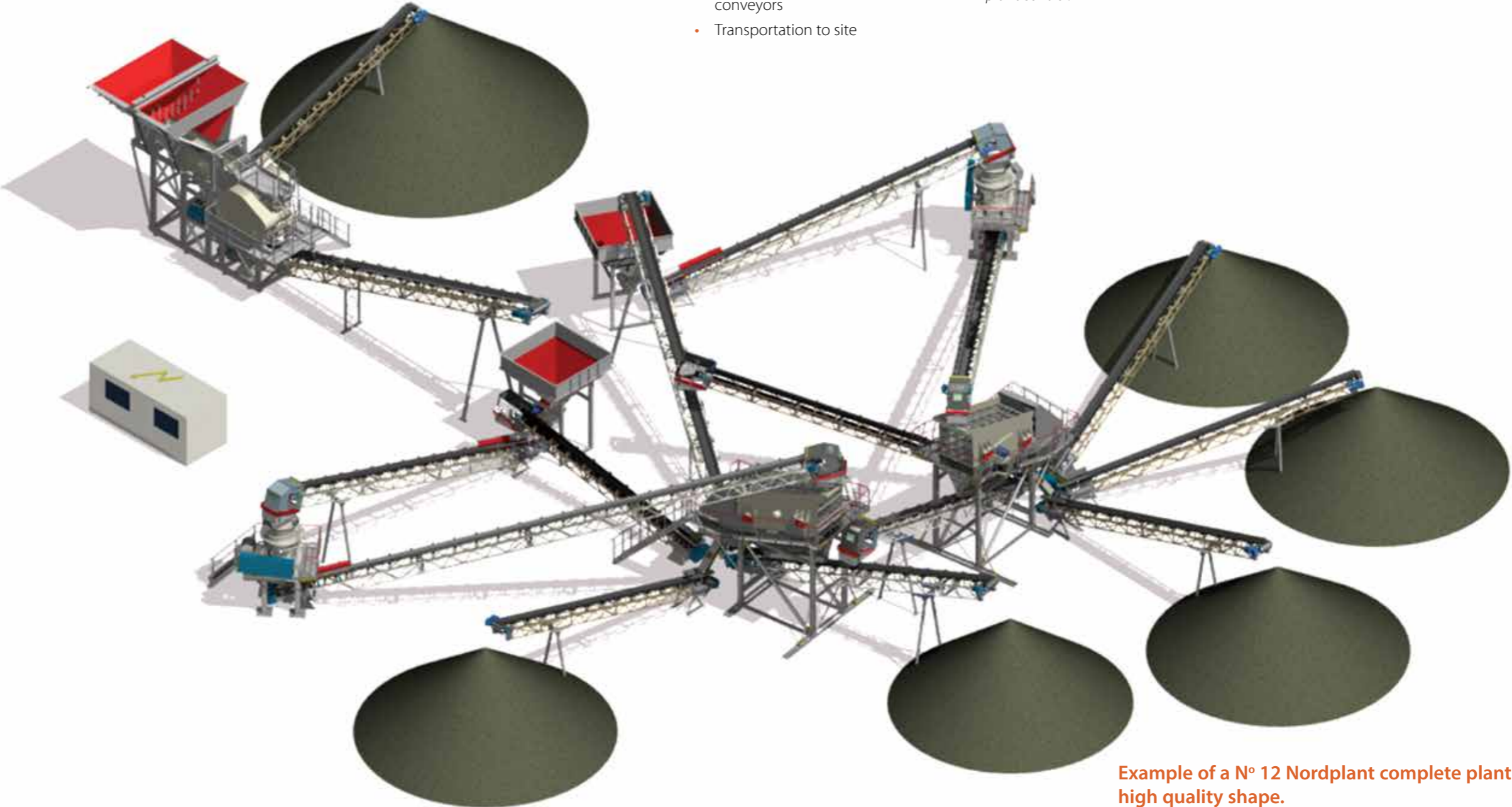
Metso's Nordplant solution includes an optional air-conditioned bungalow for electrical plant control.
